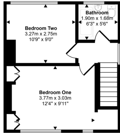
First Floor Approx 32 sq m / 342 sq ft
